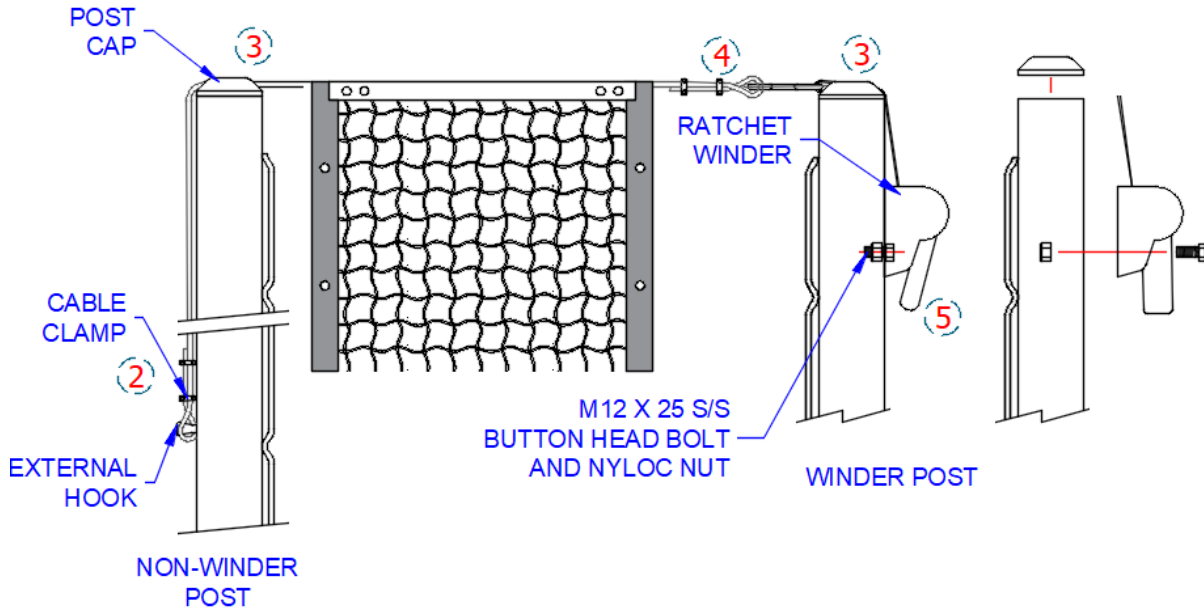
Figure 5: Net Installation Details
