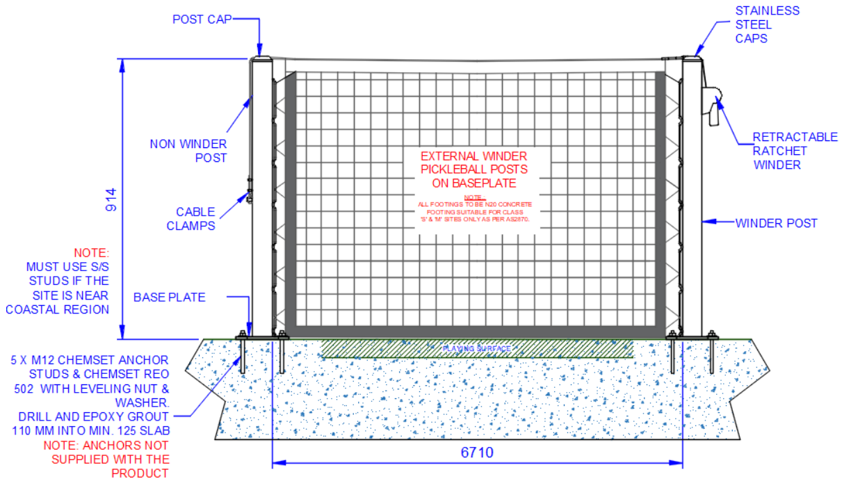
Figure 7: PBR-BP Footing and Assembly Details
