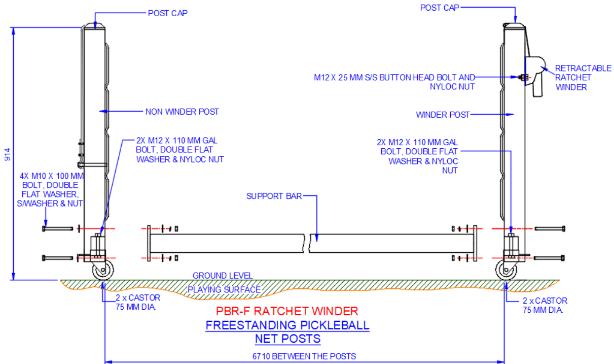
Figure 8: PBR-F Assembly Details
