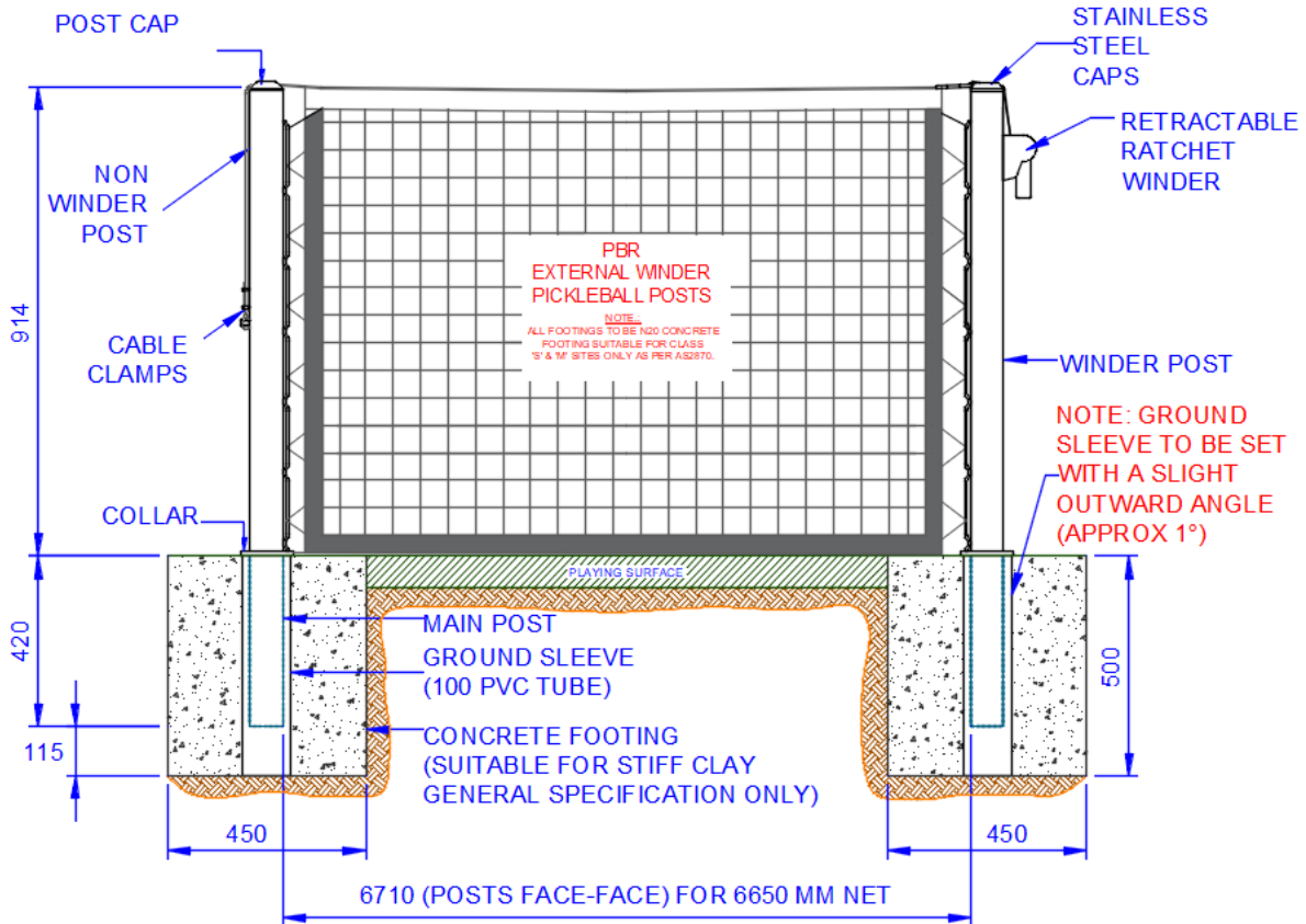
Figure 6: PBR Footing & Assembly Details
