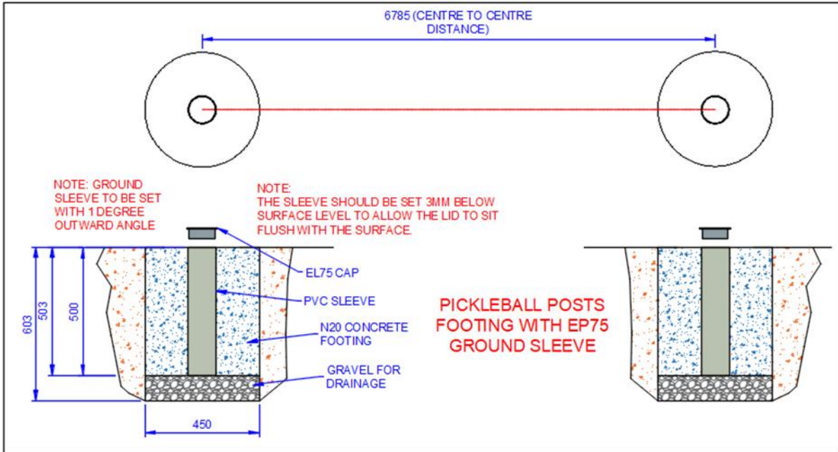
Figure 2: EP75 & EL75 Footing Details
