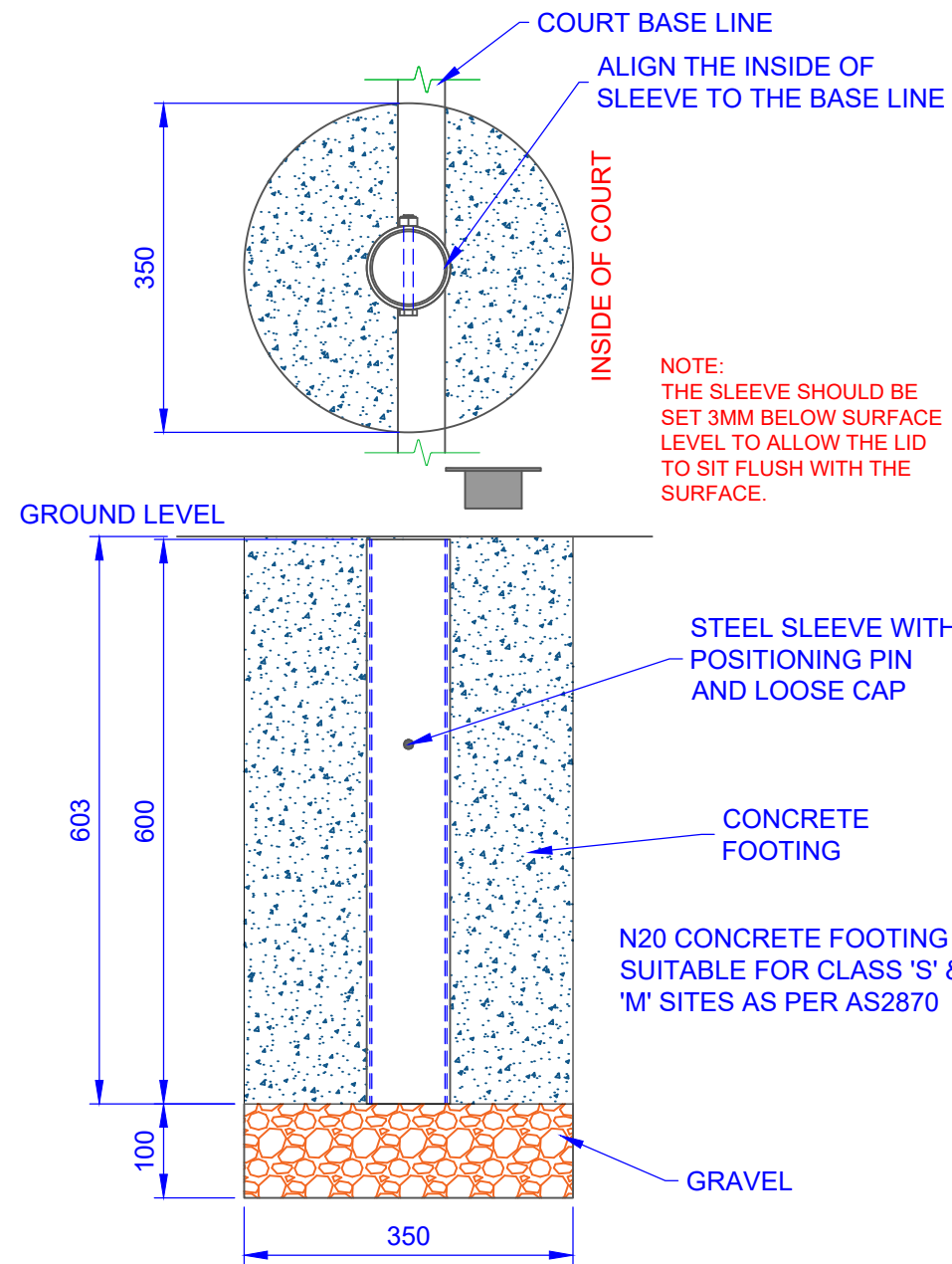
SLEEVE OPTION: ES76 PVC SLEEVE WITH EL76 LOOSE CAP
