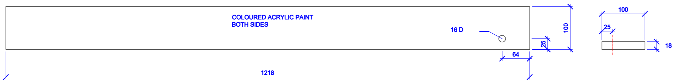
TLJ29 FLUSH TOE BOARD 18 MM MARINE PLY TOE BOARD
