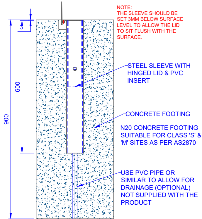
SLEEVE OPTION: EHC60s STEEL SLEEVE WITH HINGED CAP
